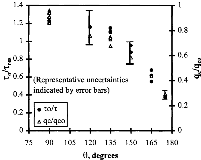
Fig. 9. Reciprocal of the measured bubble residence time as a function of heater surface orientation compared with the corresponding CHF; test conditions: U_{\text{bulk}} = 0.04 \text{ m s}^{-1} ; Re = 5400 ; T_{\text{in}} = 322 \text{ K} ; test section height = 25.4 mm.
