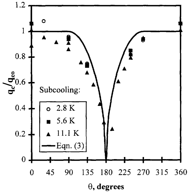
Fig. 5. Measured CHF as a function of heater surface orientation, compared with the CHF model of equation (3); test conditions: U_{bulk} = 0.04 \text{ m s}^{-1} ; Re = 2700 ; T_{in} = 322 \text{ K} .
