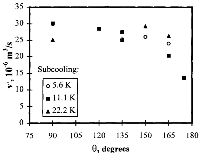
Fig. 6. Volumetric rate of vapor generation as a function of the heater surface orientation for various levels of subcooling; test conditions: U_{bulk} = 0.04 \text{ m s}^{-1} ; Re = 5400 ; T_{in} = 322 \text{ K} ; test section height = 25.4 mm.
